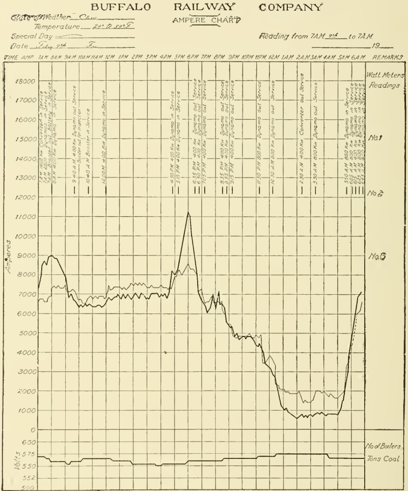
Fig. 142. Load Diagram for Large System
